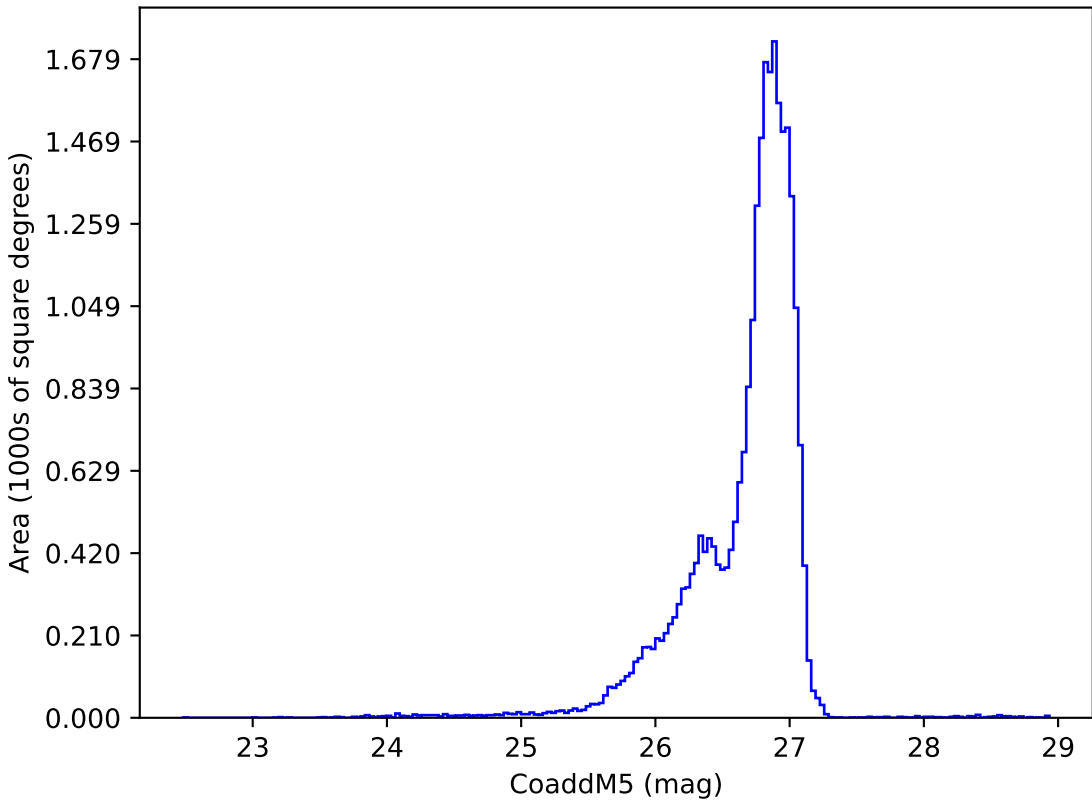
early_ss_template_fpextra2.0_v3.4_10yrs g: CoaddM5
