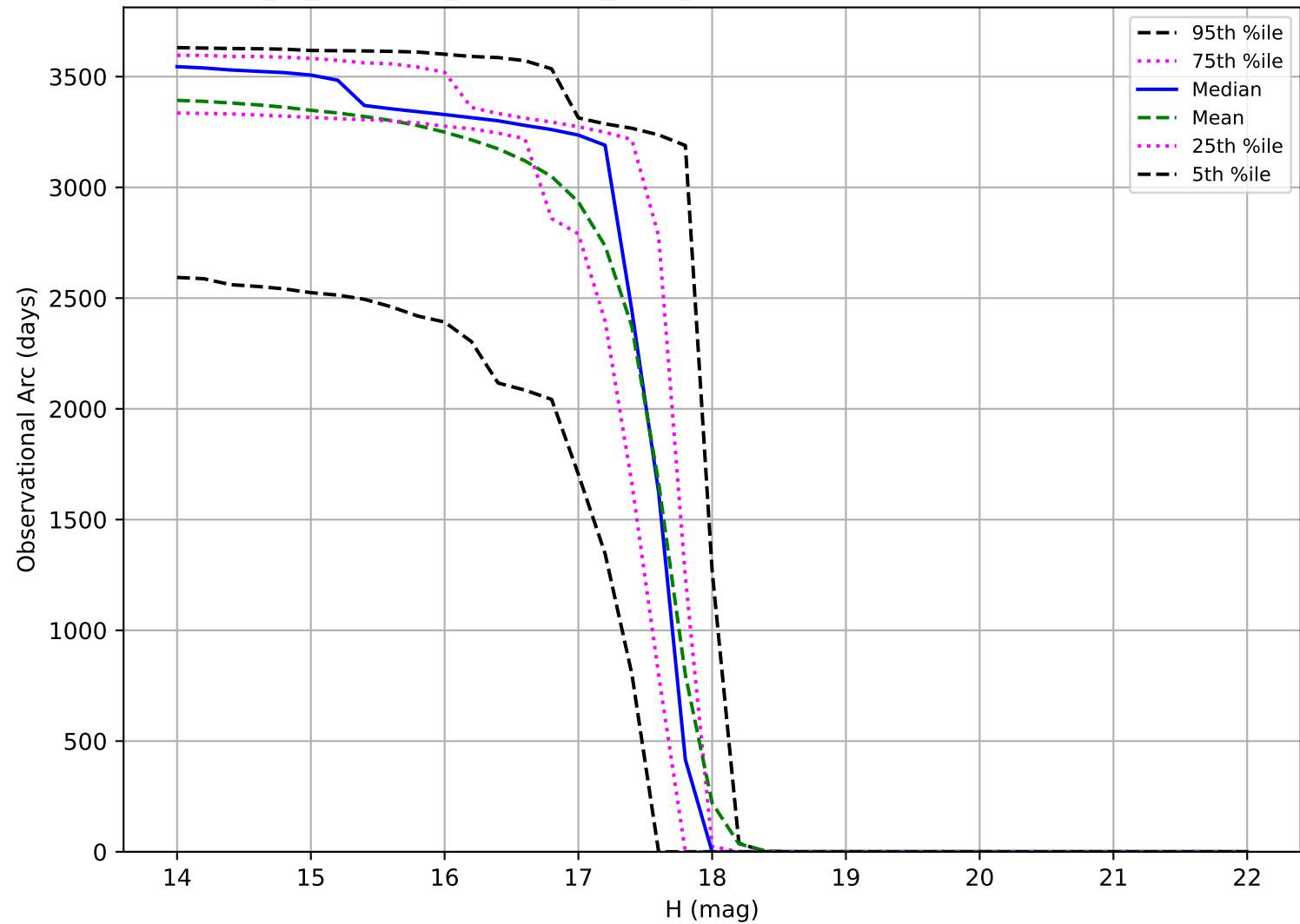
early_ss_template_fpextra1.5_v3.4_10yrs: Observational Arc Length Trojan
