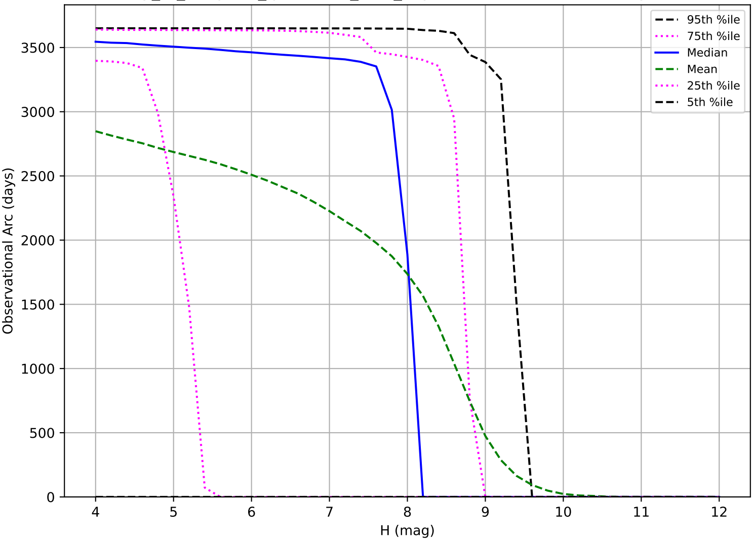
early_ss_template_fpextra1.5_v3.4_10yrs: Observational Arc Length TNO
