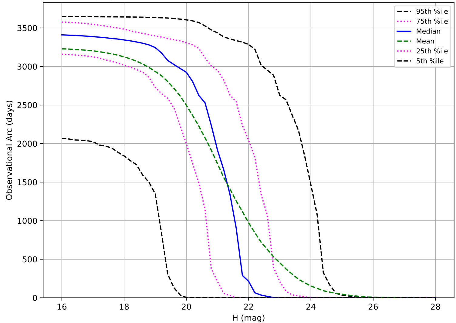
early_ss_template_fpextra1.5_v3.4_10yrs: Observational Arc Length PHA
