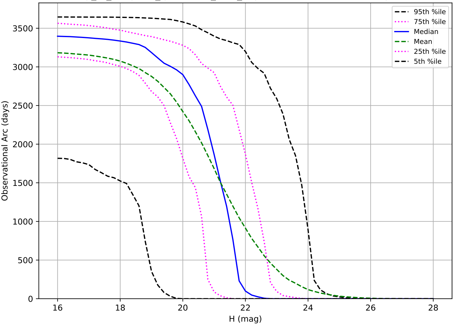
early_ss_template_fpextra1.5_v3.4_10yrs: Observational Arc Length NEO
