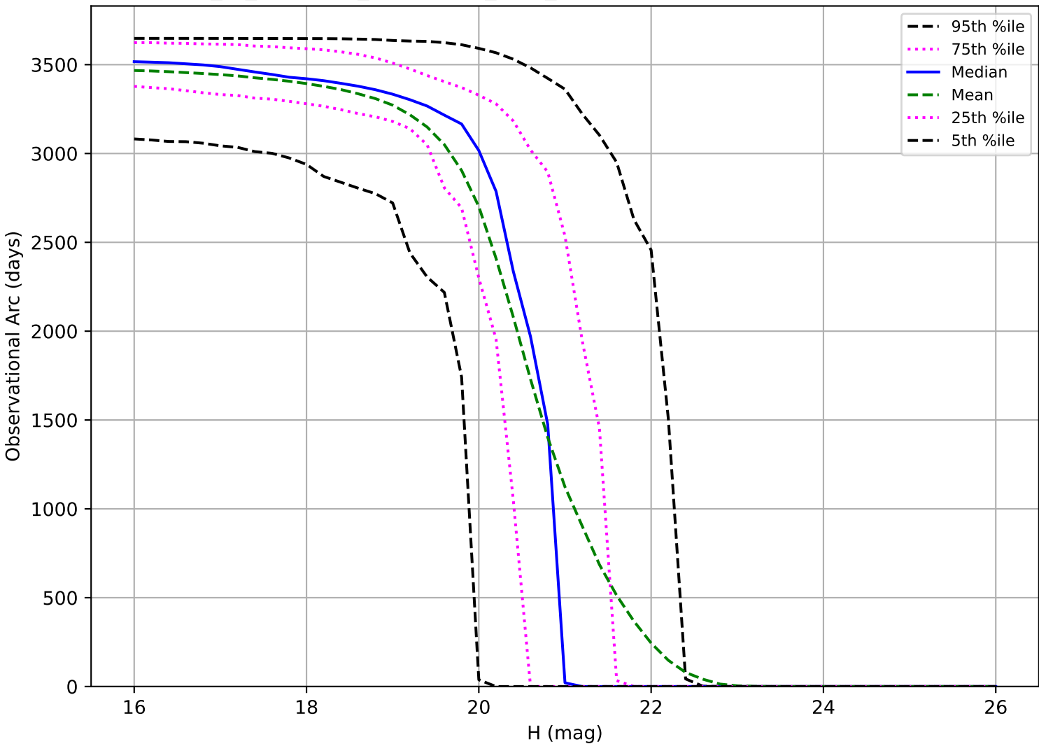
early_ss_template_fpextra1.5_v3.4_10yrs: Observational Arc Length MBA
