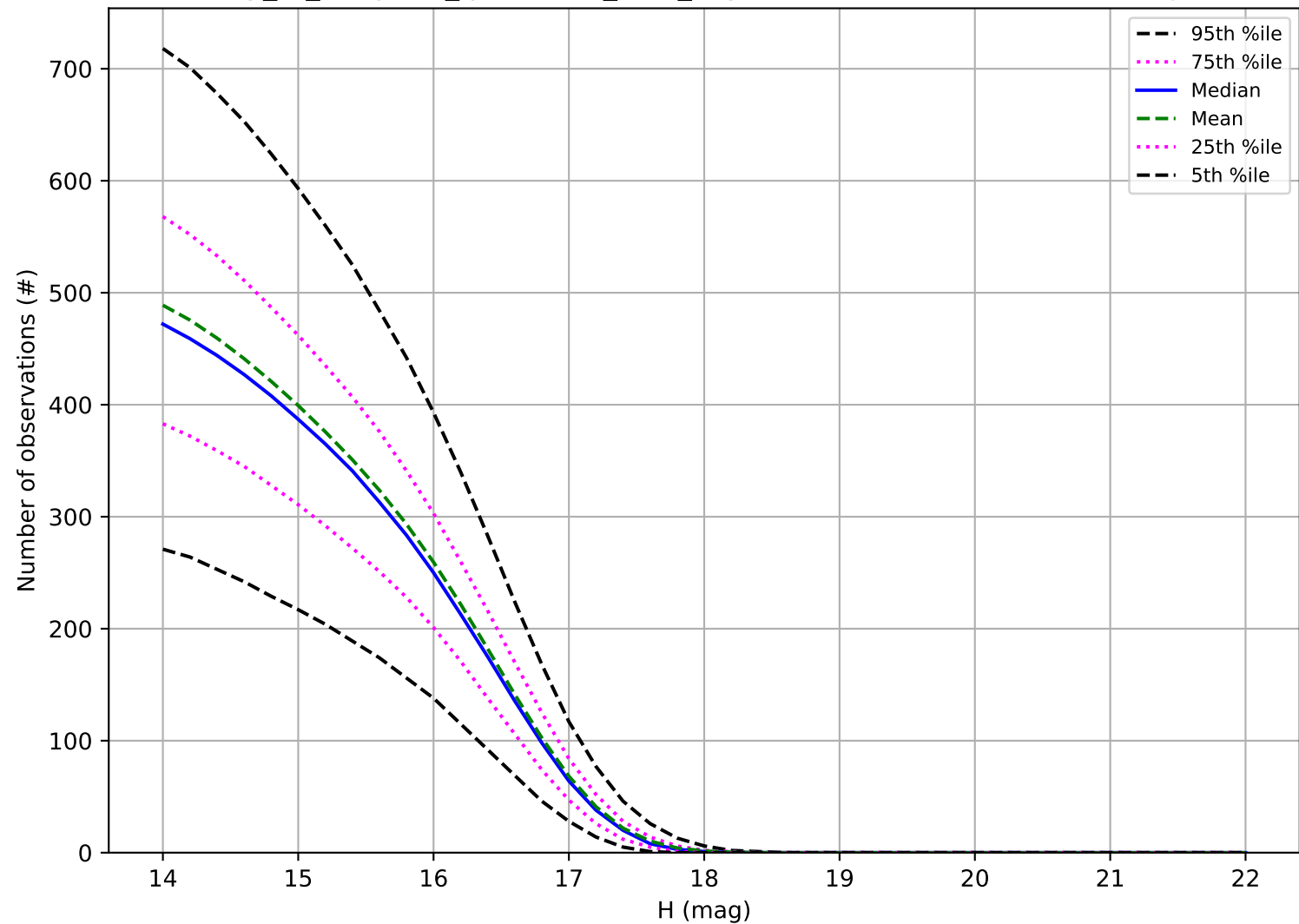
early_ss_template_fpextra1.5_v3.4_10yrs: Number of observations Trojan
