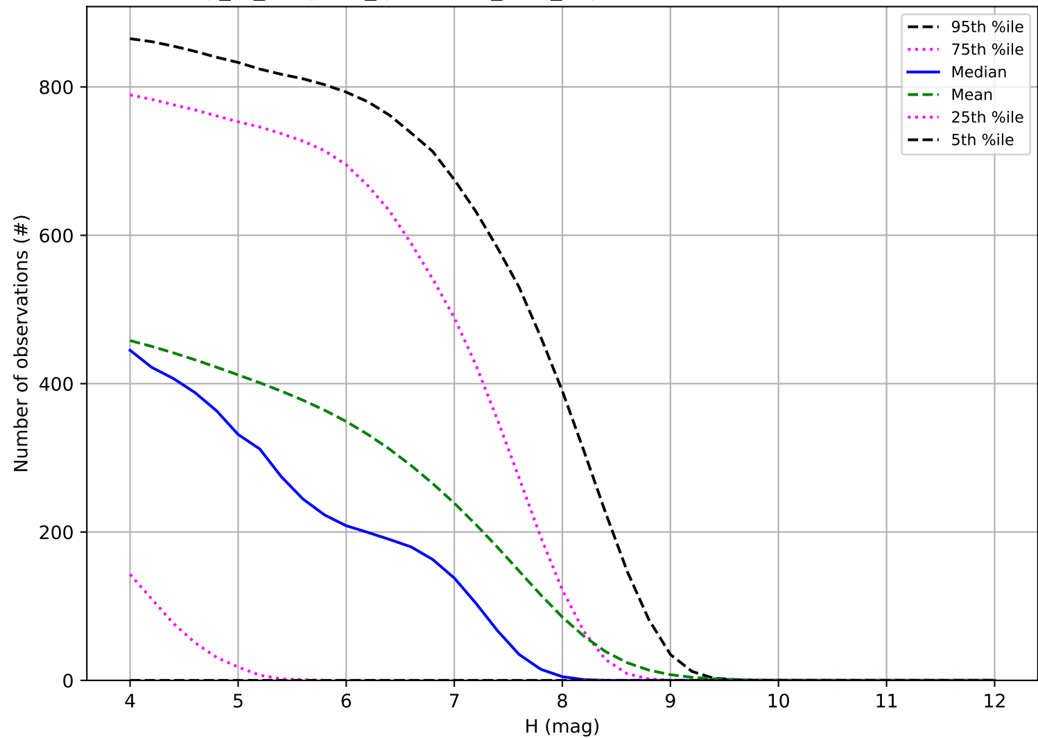
early_ss_template_fpextra1.5_v3.4_10yrs: Number of observations TNO
