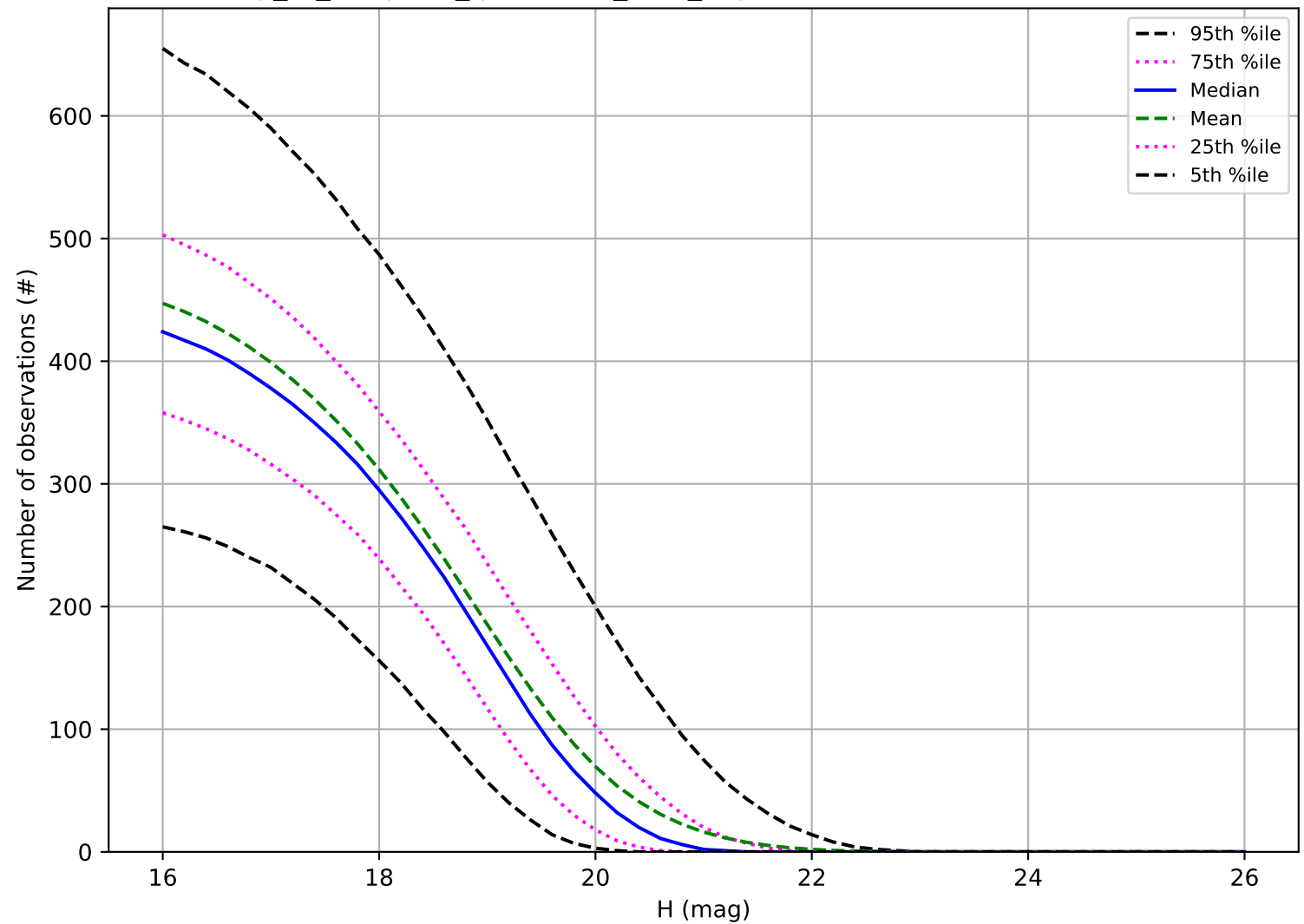
early_ss_template_fpextra1.5_v3.4_10yrs: Number of observations MBA
