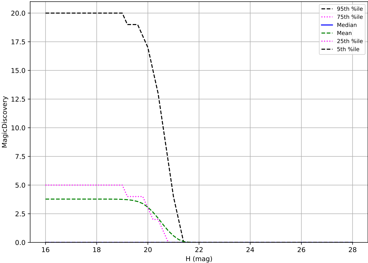
early_ss_template_fpextra1.5_v3.4_10yrs: Vatira 6 detections in 60 nights detection loss
