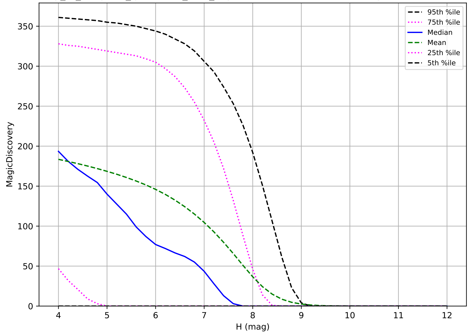
early_ss_template_fpextra1.5_v3.4_10yrs: TNO 6 detections in 60 nights detection loss
