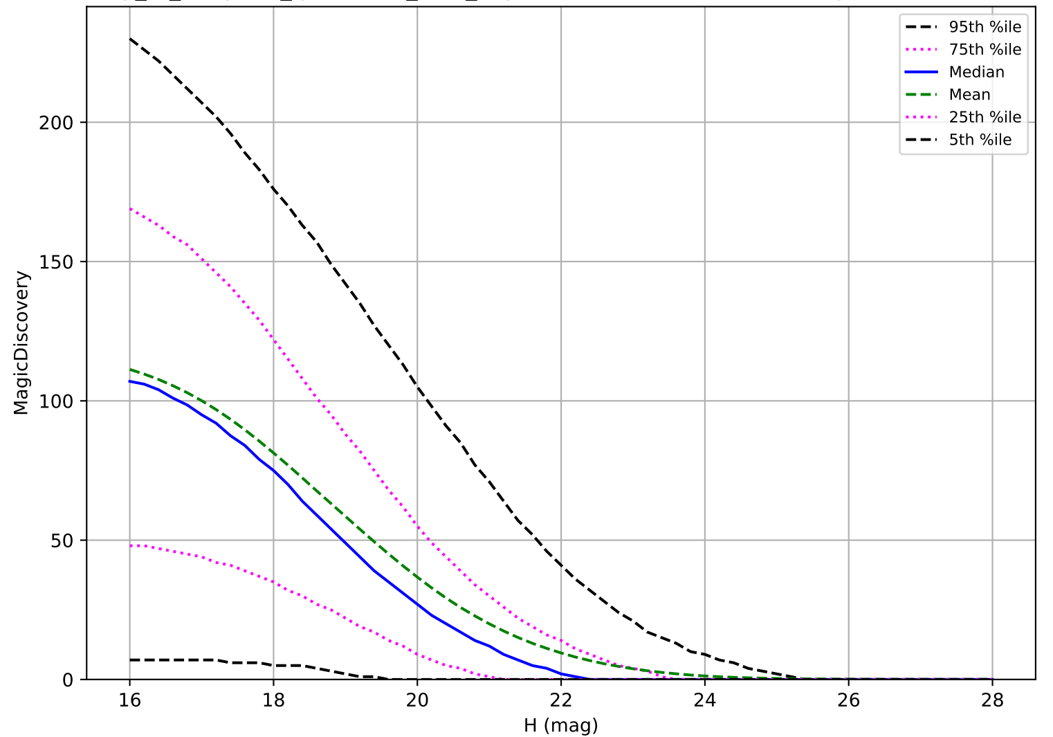
early_ss_template_fpextra1.5_v3.4_10yrs: PHA 6 detections in 60 nights detection loss
