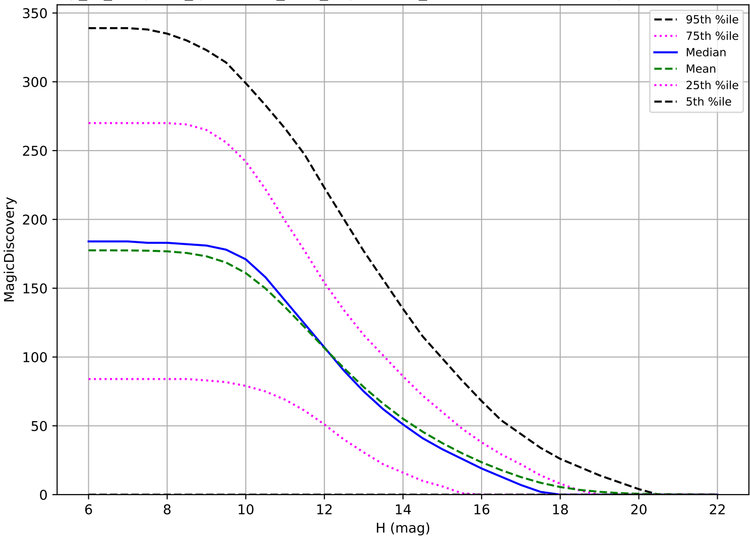
early_ss_template_fpextra1.5_v3.4_10yrs: OCC_r5 6 detections in 60 nights detection loss
