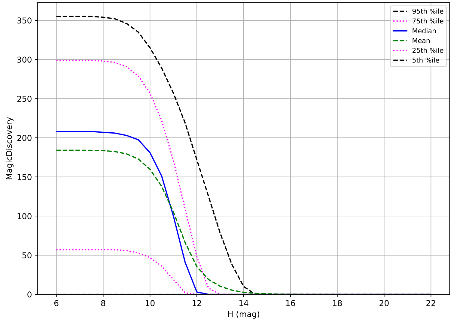
early_ss_template_fpextra1.5_v3.4_10yrs: OCC_r20 6 detections in 60 nights detection loss
