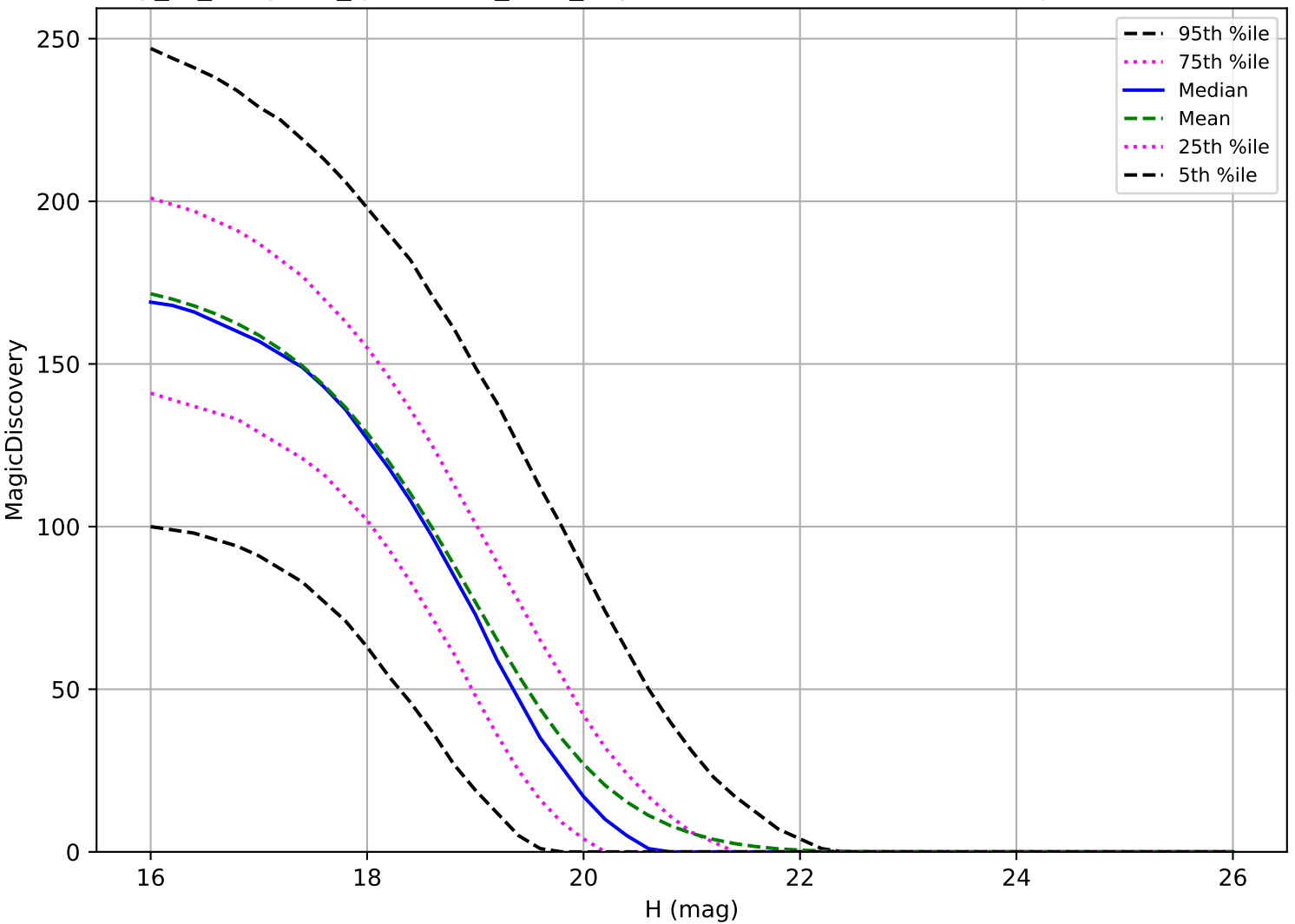
early_ss_template_fpextra1.5_v3.4_10yrs: MBA 6 detections in 60 nights detection loss
