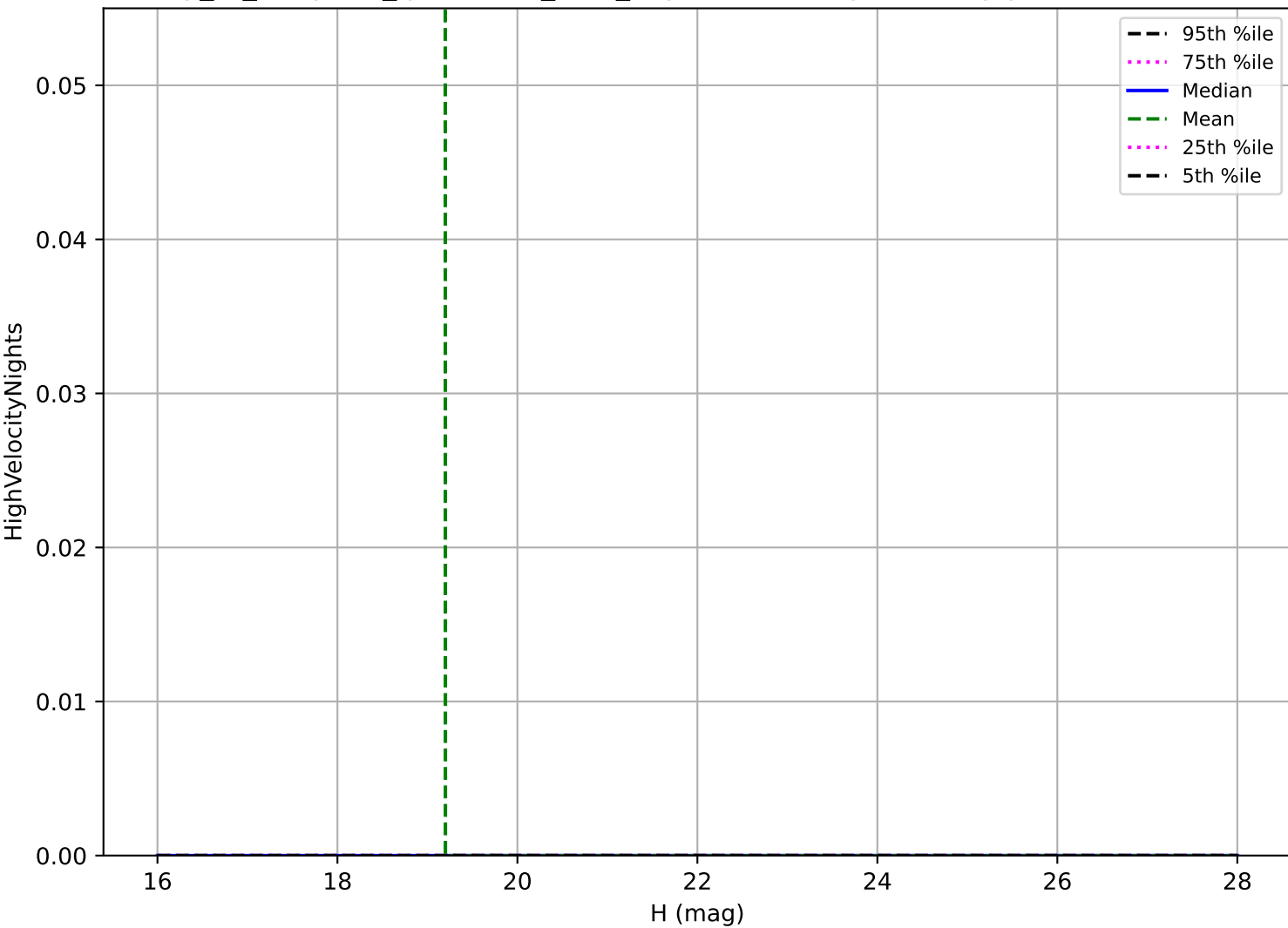
early_ss_template_fpextra1.5_v3.4_10yrs: Vatira High velocity pair detection loss
