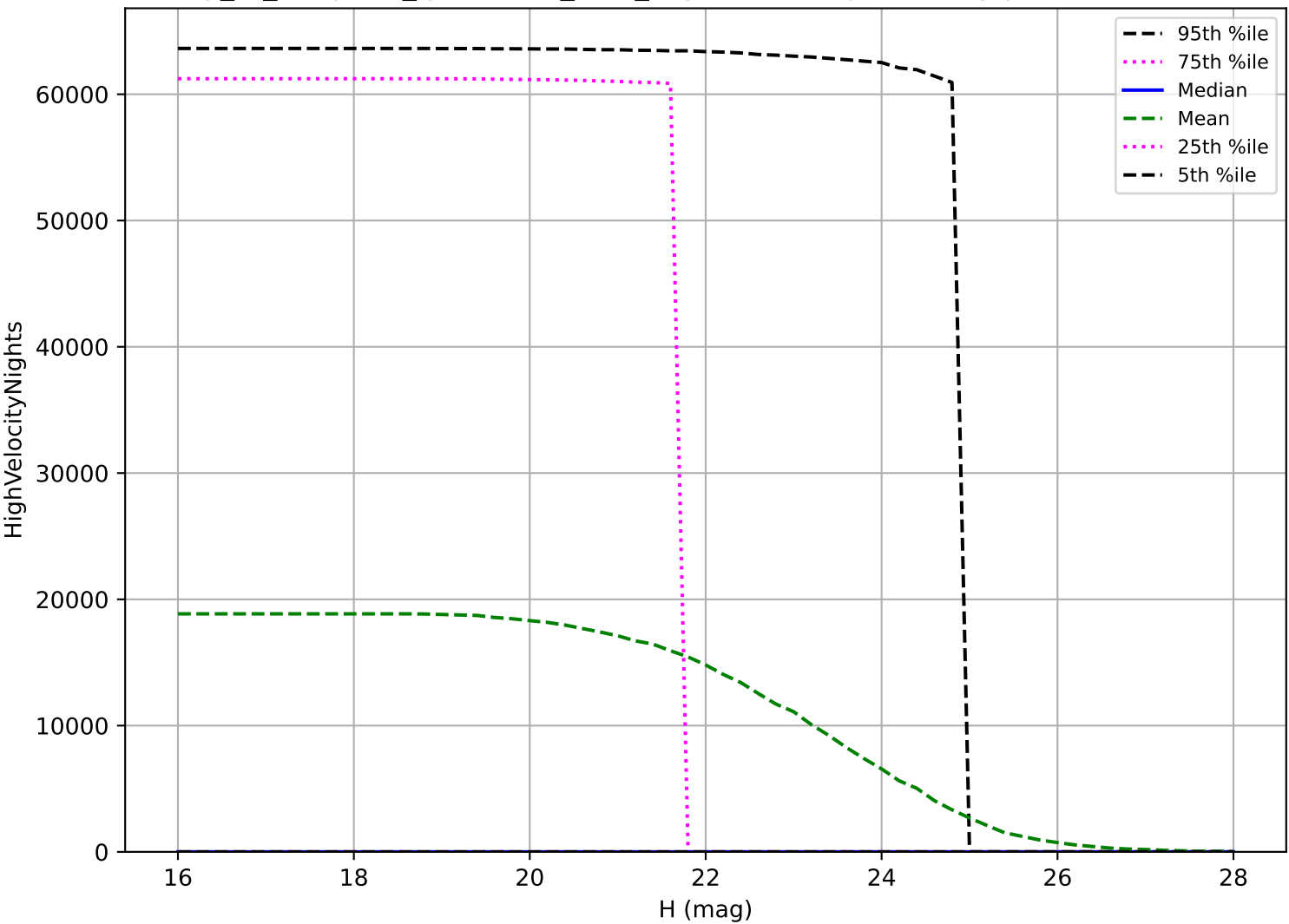
early_ss_template_fpextra1.5_v3.4_10yrs: NEO High velocity pair detection loss
