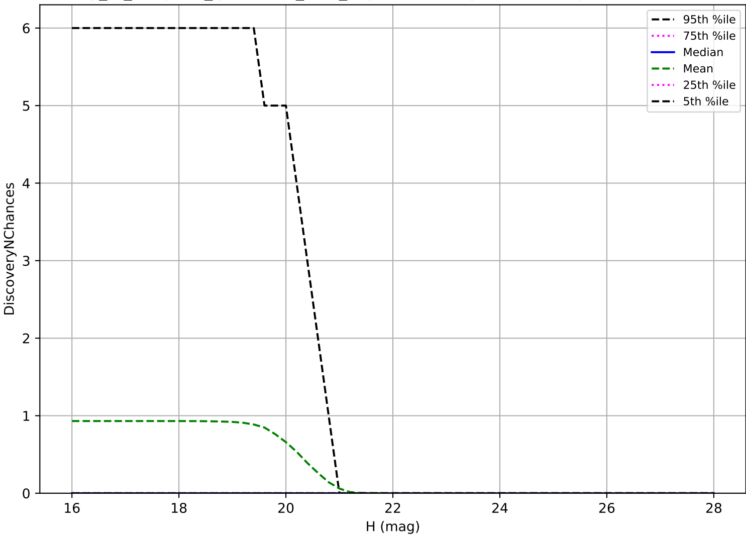
early_ss_template_fpextra1.5_v3.4_10yrs: Vatira 3 pairs in 15 nights detection loss
