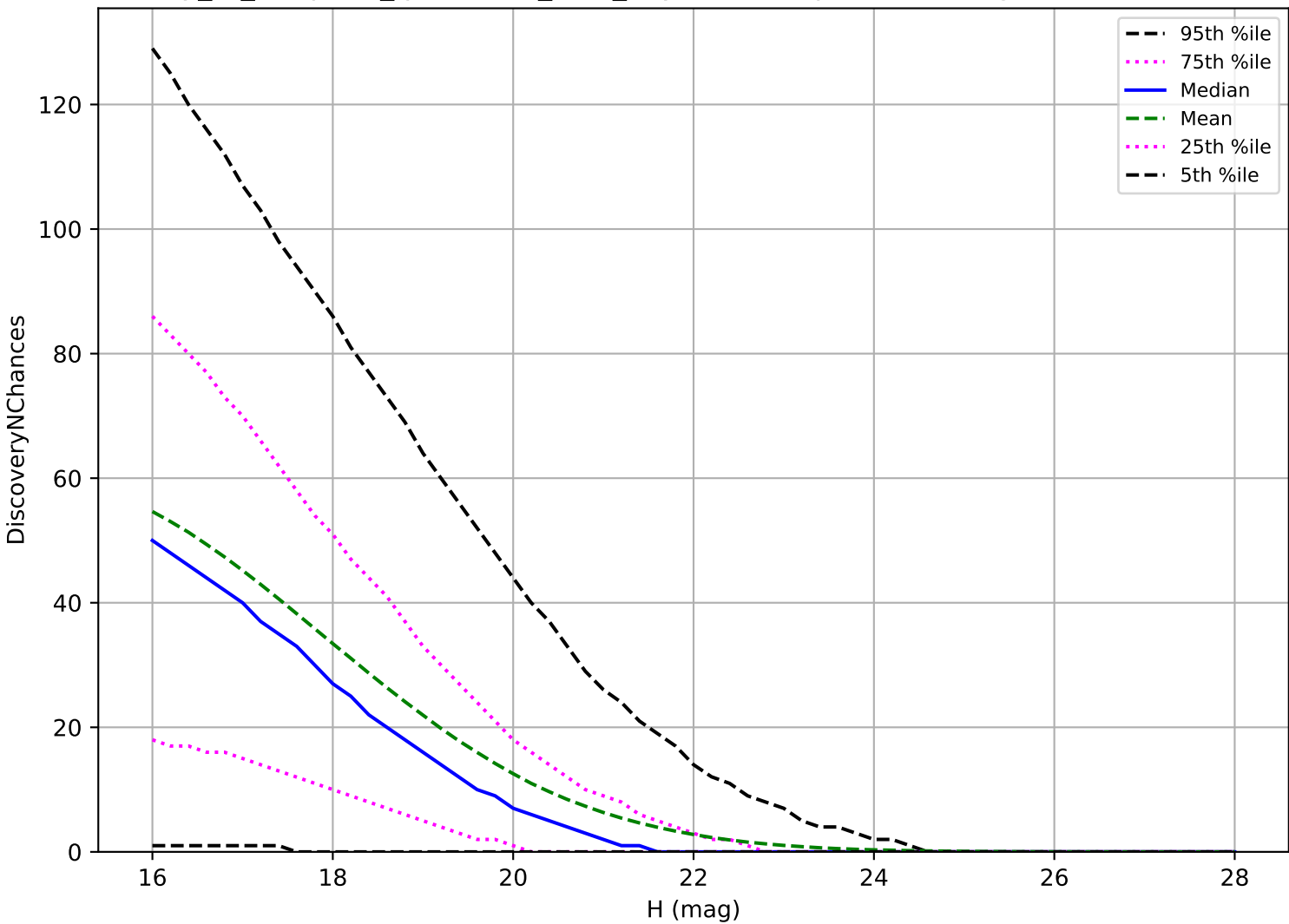
early_ss_template_fpextra1.5_v3.4_10yrs: PHA 3 pairs in 15 nights detection loss
