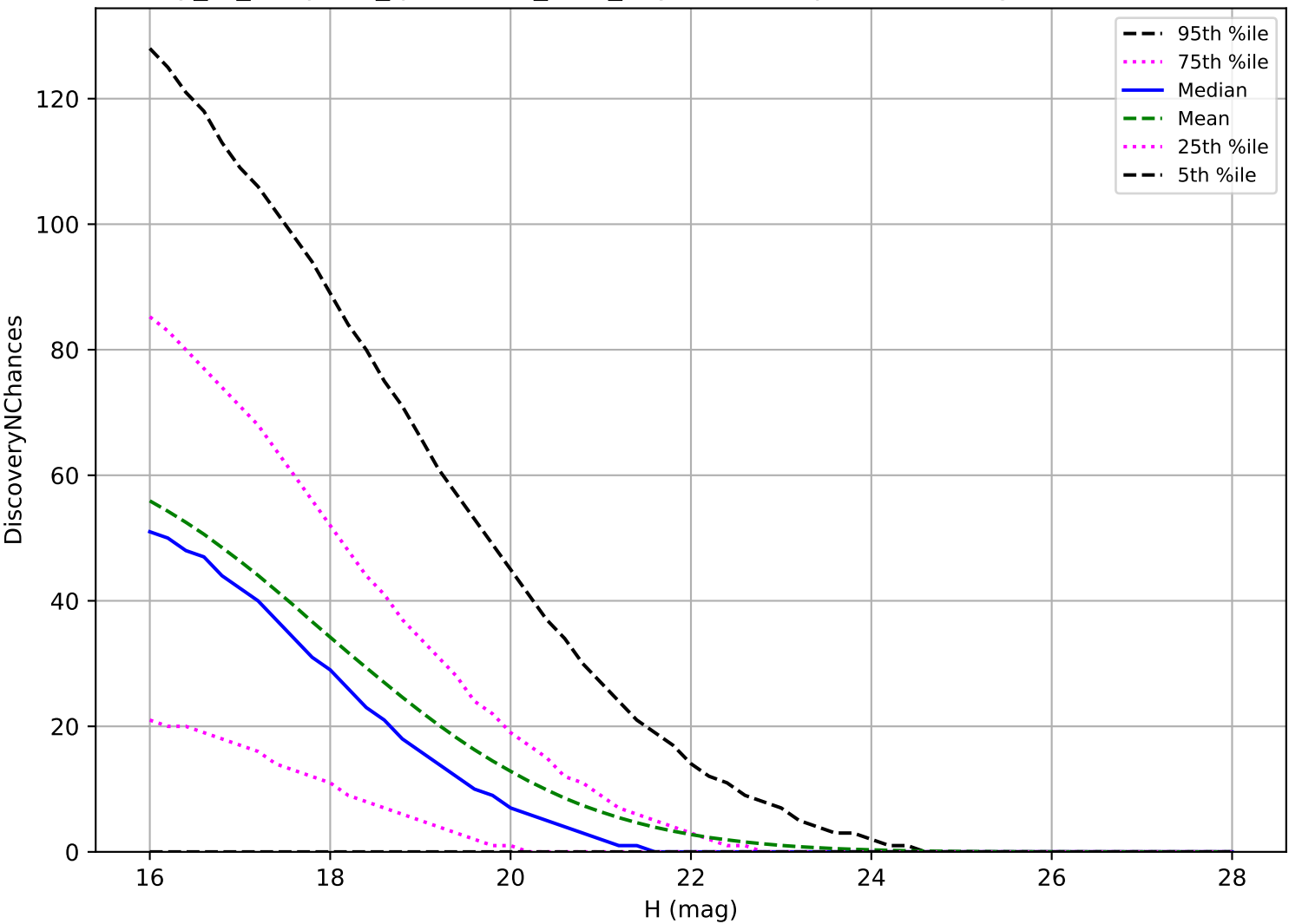
early_ss_template_fpextra1.5_v3.4_10yrs: NEO 3 pairs in 15 nights detection loss
