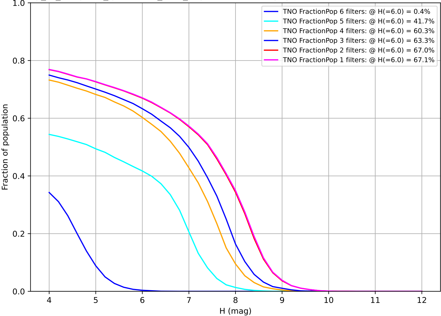
early_ss_template_fpextra1.5_v3.4_10yrs: Fraction of population with colors in X filters TNO
