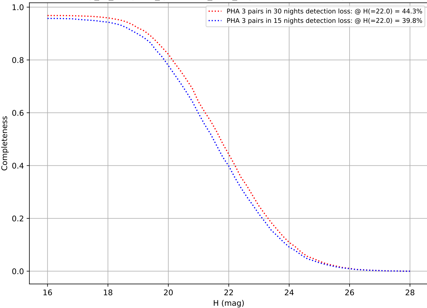
early_ss_template_fpextra1.5_v3.4_10yrs: DifferentialCompleteness
