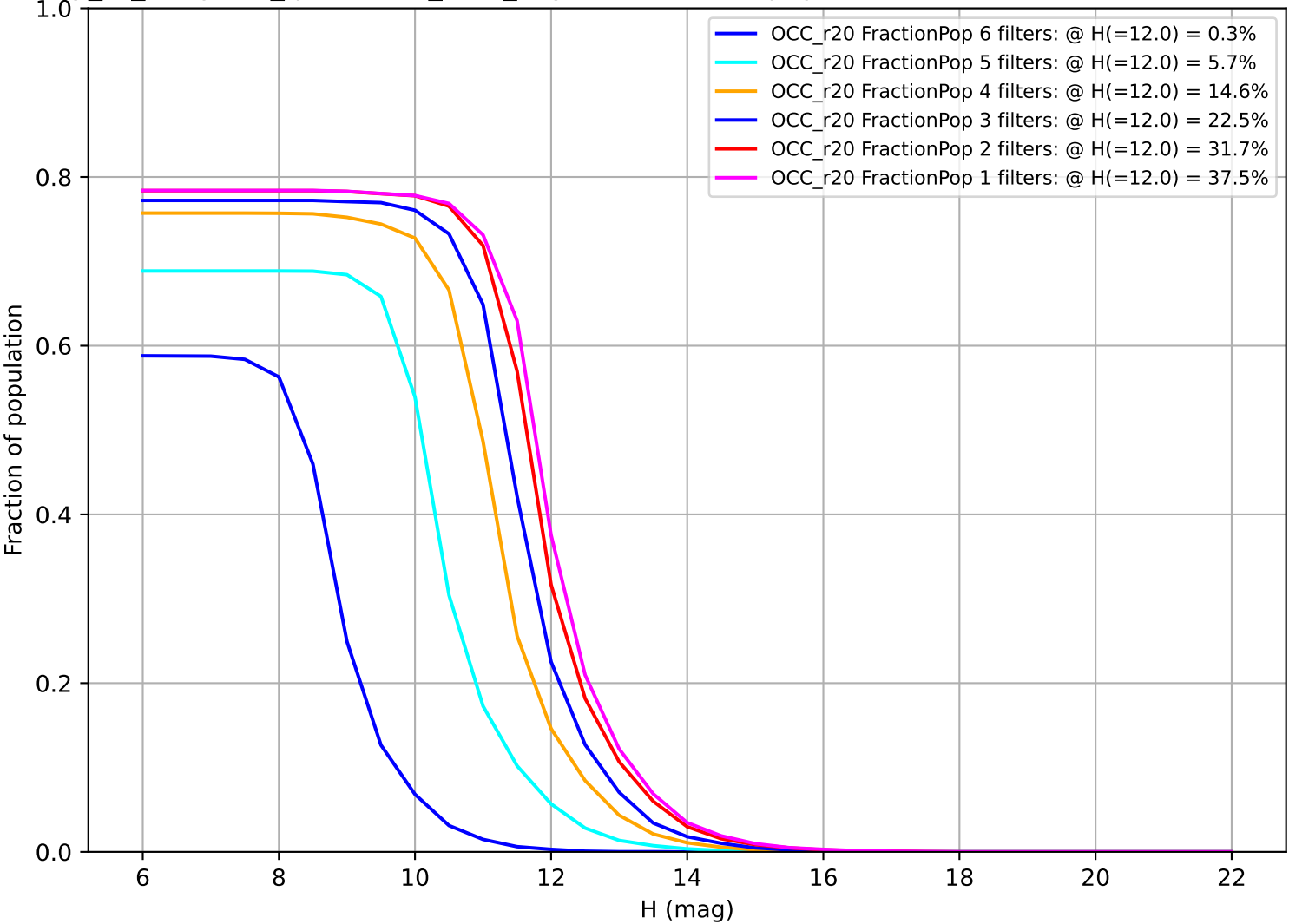
early_ss_template_fpextra1.5_v3.4_10yrs: Fraction of population with colors in X filters OCC_r20
