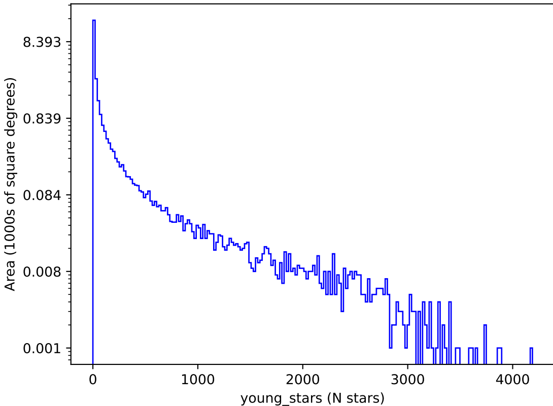
early_ss_template_fpextra1.5_v3.4_10yrs : young_stars
