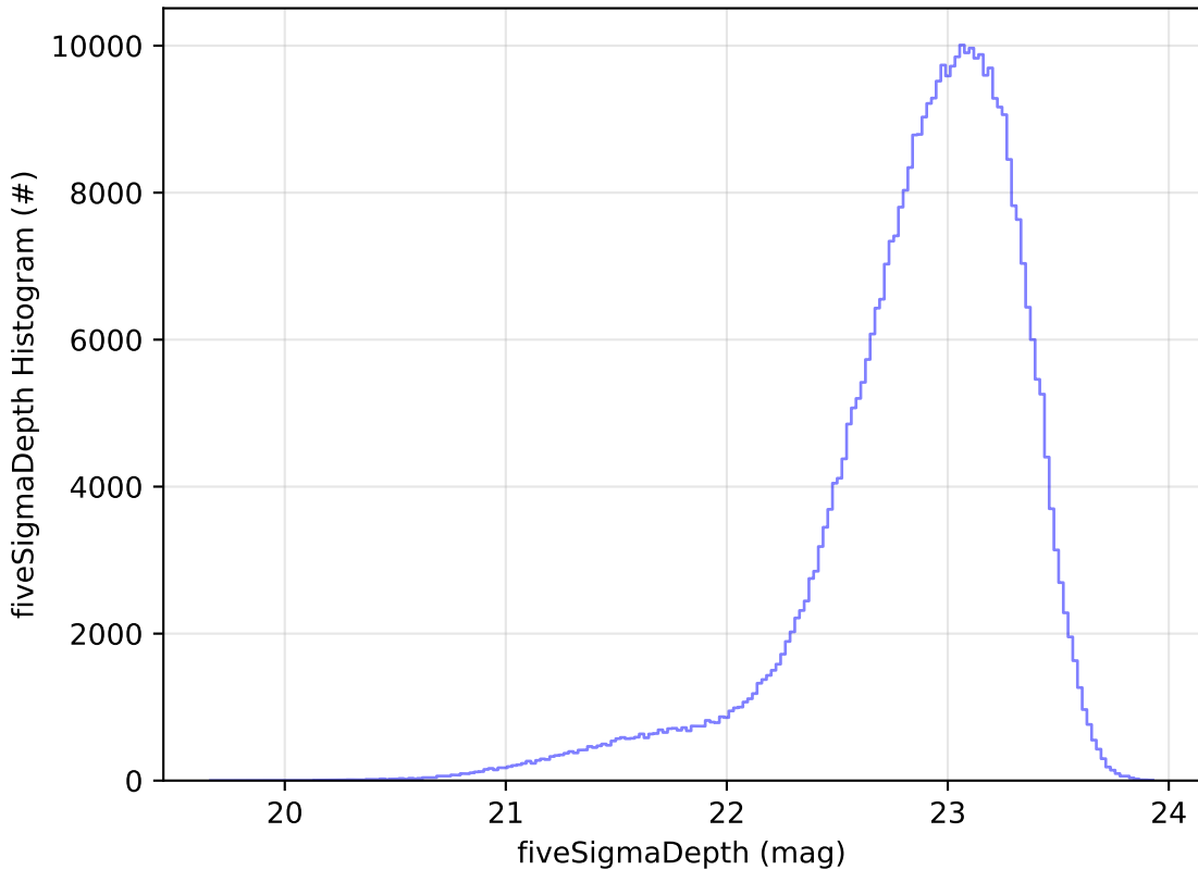
early_ss_template_fpextra1.5_v3.4_10yrs z: fiveSigmaDepth Histogram
