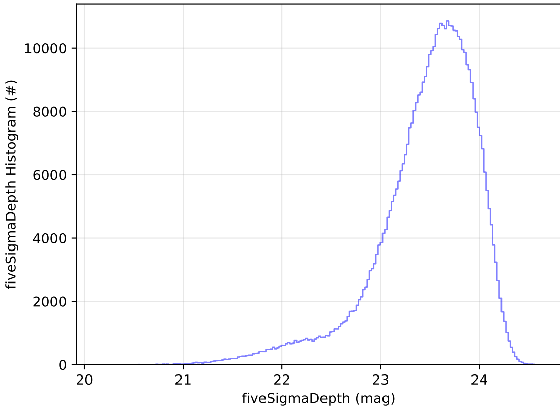
early_ss_template_fpextra1.5_v3.4_10yrs i: fiveSigmaDepth Histogram
