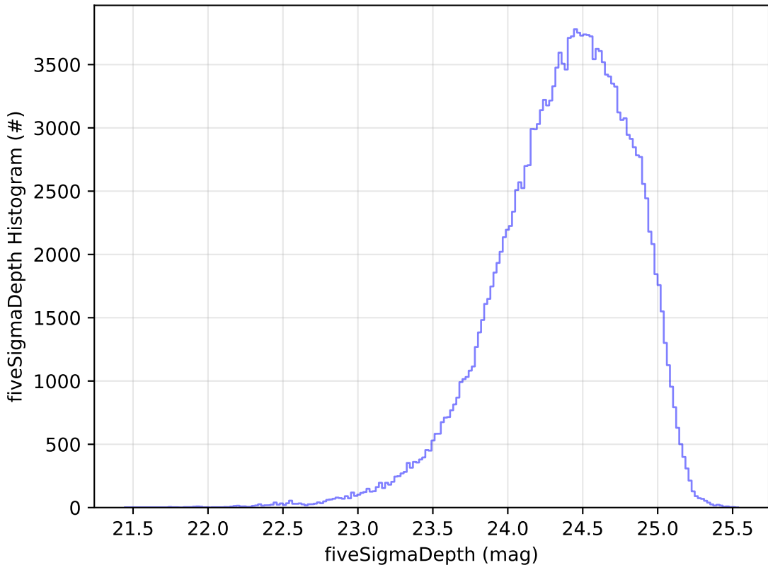
early_ss_template_fpextra1.5_v3.4_10yrs g: fiveSigmaDepth Histogram
