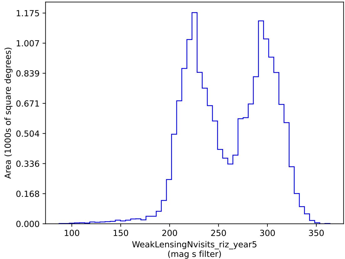
early_ss_template_fpextra1.5_v3.4_10yrs gri band non-DD: WeakLensingNvisits_riz_year5
