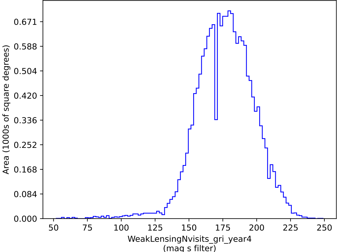
early_ss_template_fpextra1.5_v3.4_10yrs gri band non-DD: WeakLensingNvisits_gri_year4
