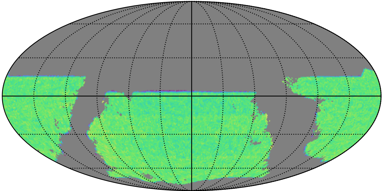
early_ss_template_fpextra1.5_v3.4_10yrs gri band non-DD: WeakLensingNvisits
