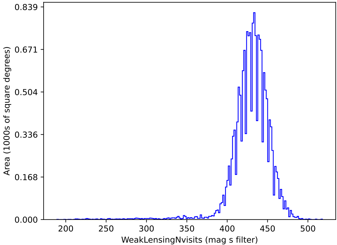
early_ss_template_fpextra1.5_v3.4_10yrs gri band non-DD: WeakLensingNvisits
