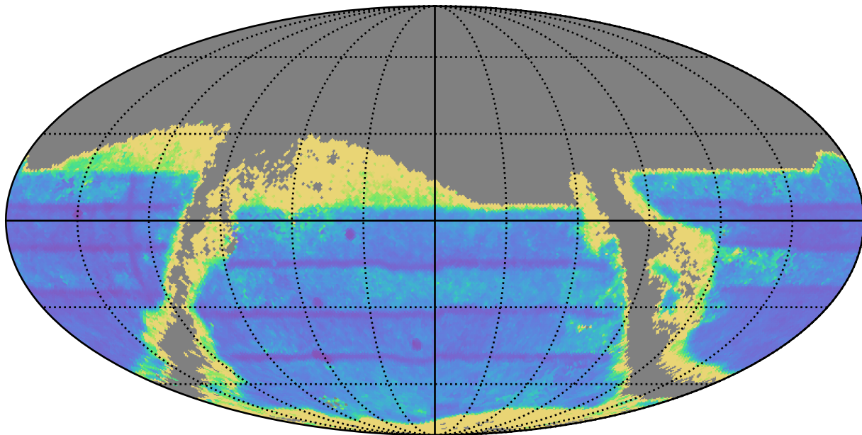
early_ss_template_fpextra1.5_v3.4_10yrs : TDC_precision
