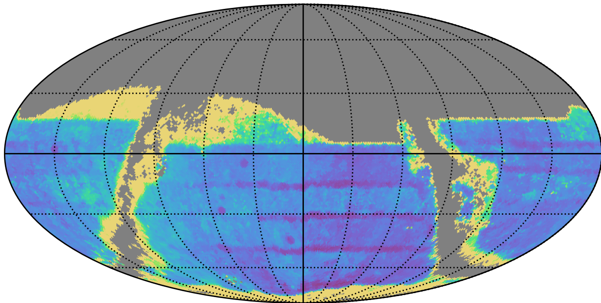
early_ss_template_fpextra1.5_v3.4_10yrs : TDC_accuracy
