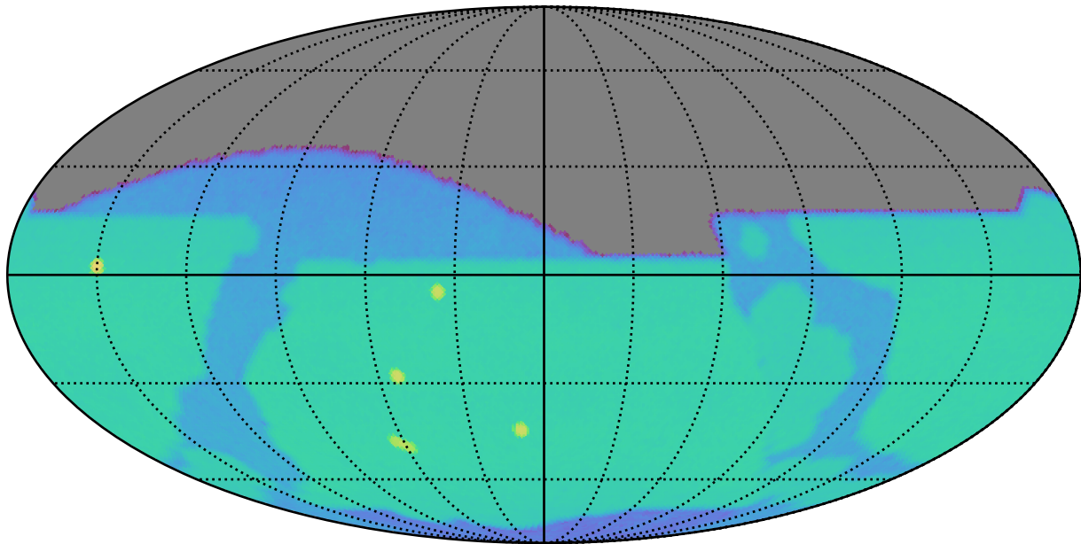
early_ss_template_fpextra1.5_v3.4_10yrs z: SurfaceBrightLimit
