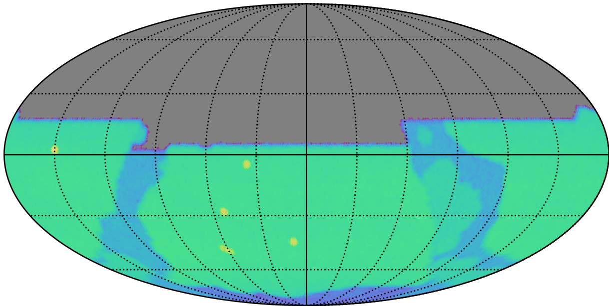
early_ss_template_fpextra1.5_v3.4_10yrs y: SurfaceBrightLimit
