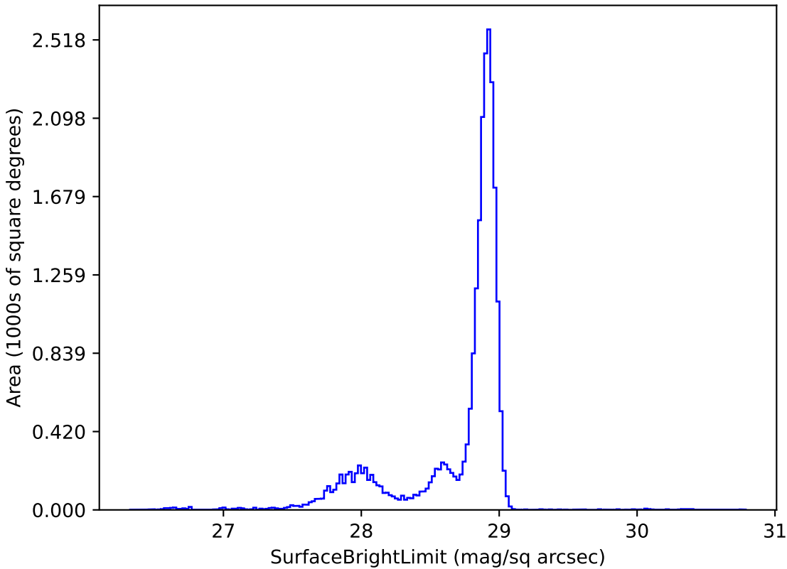
early_ss_template_fpextra1.5_v3.4_10yrs u: SurfaceBrightLimit
