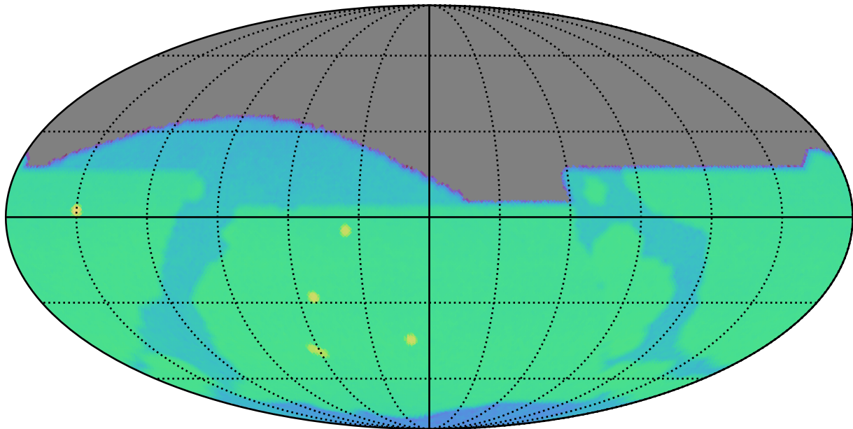
early_ss_template_fpextra1.5_v3.4_10yrs r: SurfaceBrightLimit
