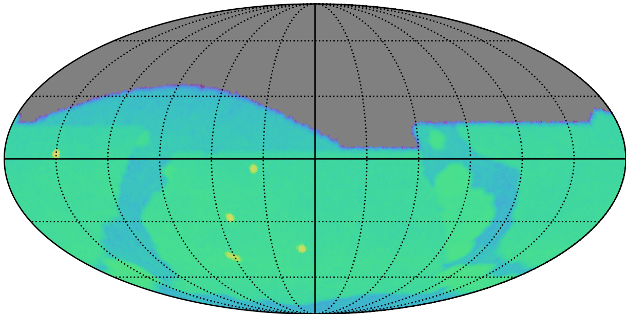
early_ss_template_fpextra1.5_v3.4_10yrs g: SurfaceBrightLimit
