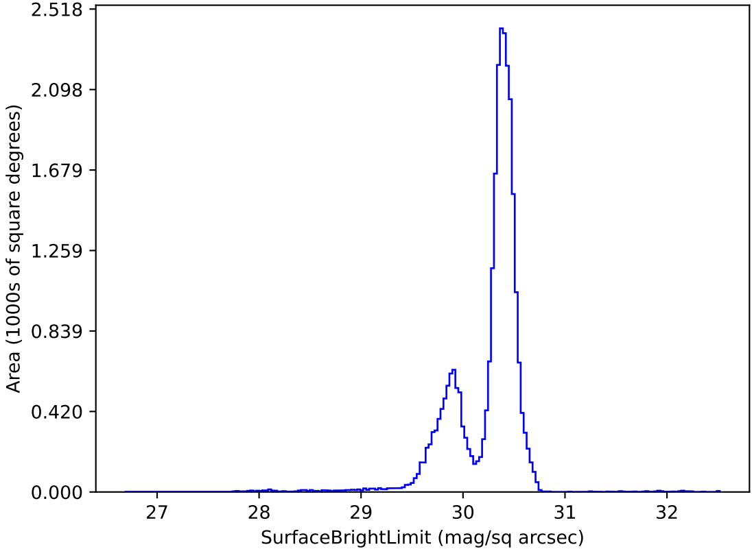
early_ss_template_fpextra1.5_v3.4_10yrs g: SurfaceBrightLimit
