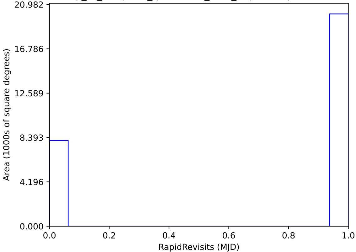
early_ss_template_fpextra1.5_v3.4_10yrs : RapidRevisits
