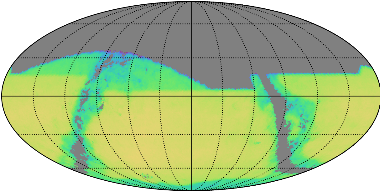
early_ss_template_fpextra1.5_v3.4_10yrs z band and non-DD: QSONumberCountsMetric
