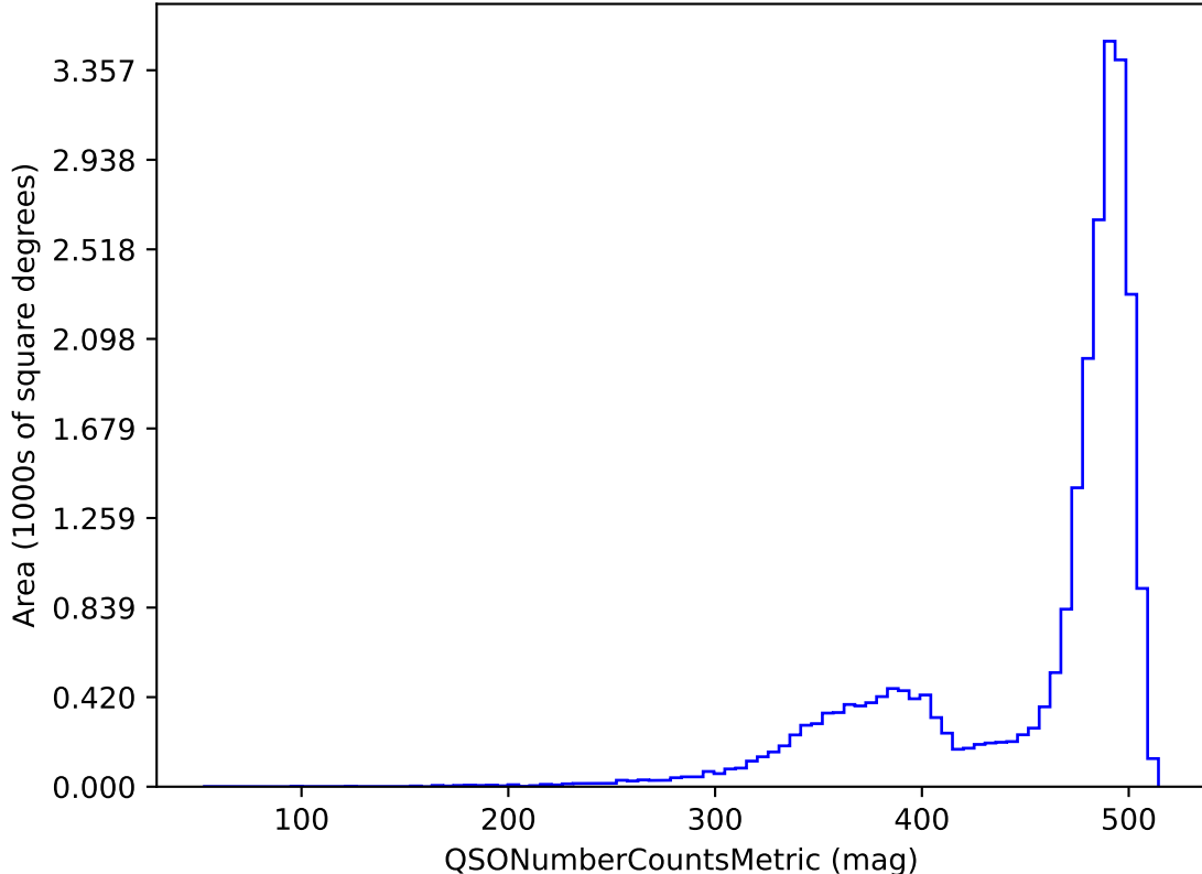
early_ss_template_fpextra1.5_v3.4_10yrs z band and non-DD: QSONumberCountsMetric
