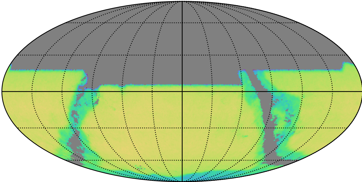
early_ss_template_fpextra1.5_v3.4_10yrs y band and non-DD: QSONumberCountsMetric
