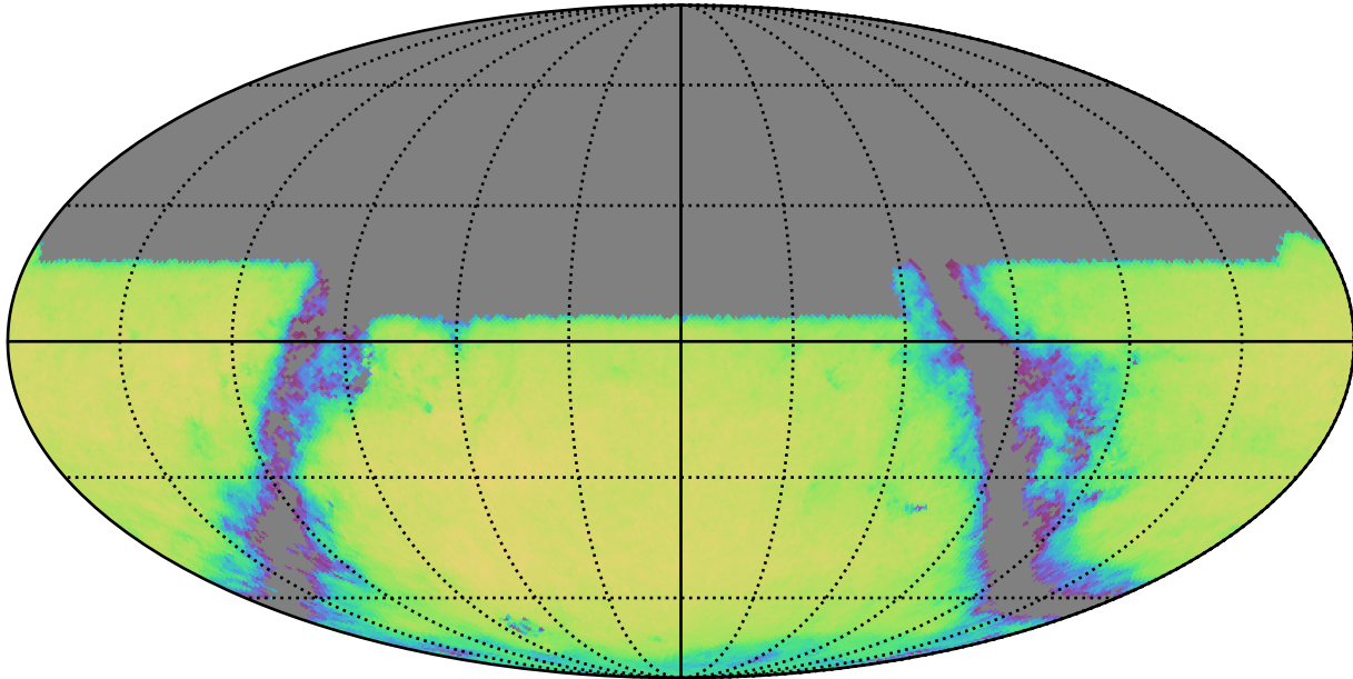
early_ss_template_fpextra1.5_v3.4_10yrs u band and non-DD: QSONumberCountsMetric
