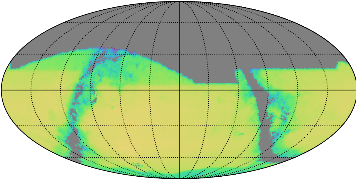
early_ss_template_fpextra1.5_v3.4_10yrs r band and non-DD: QSONumberCountsMetric
