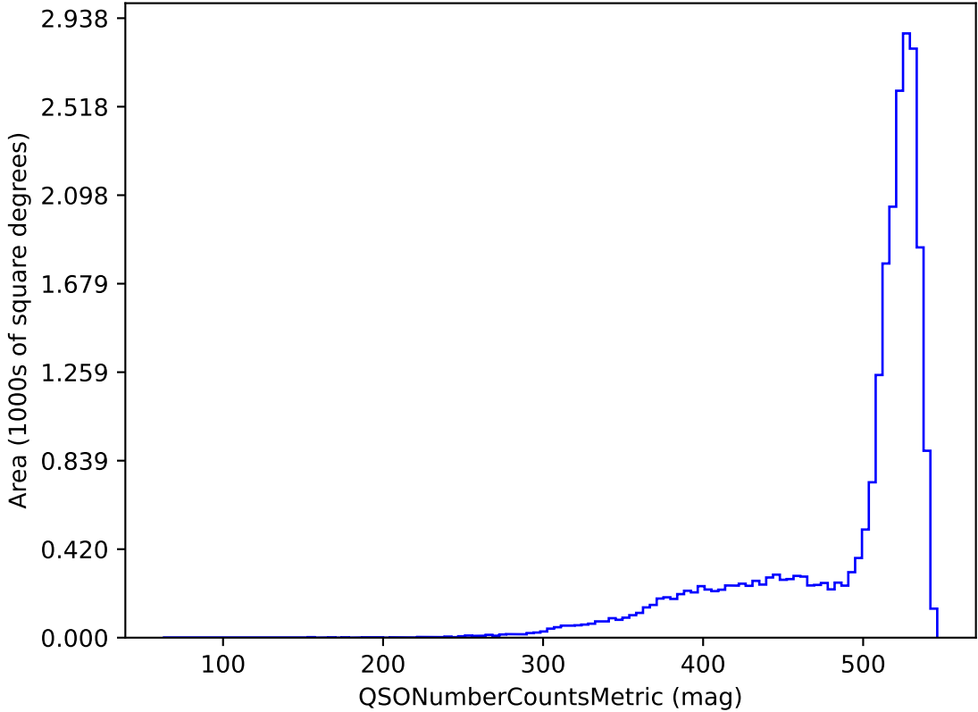
early_ss_template_fpextra1.5_v3.4_10yrs r band and non-DD: QSONumberCountsMetric
