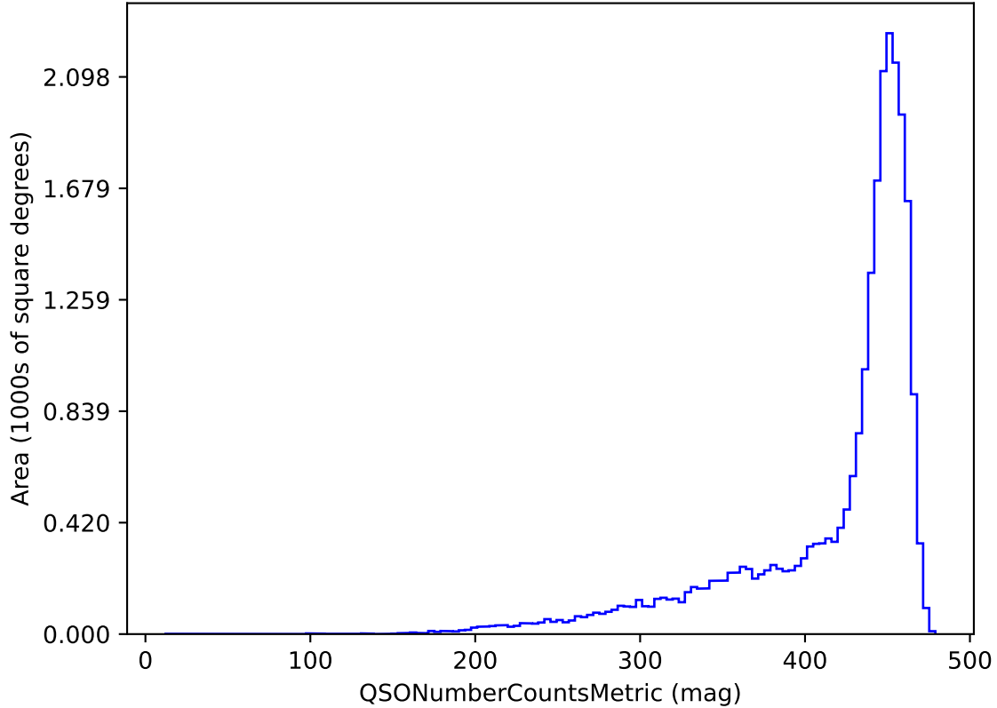
early_ss_template_fpextra1.5_v3.4_10yrs g band and non-DD: QSONumberCountsMetric
