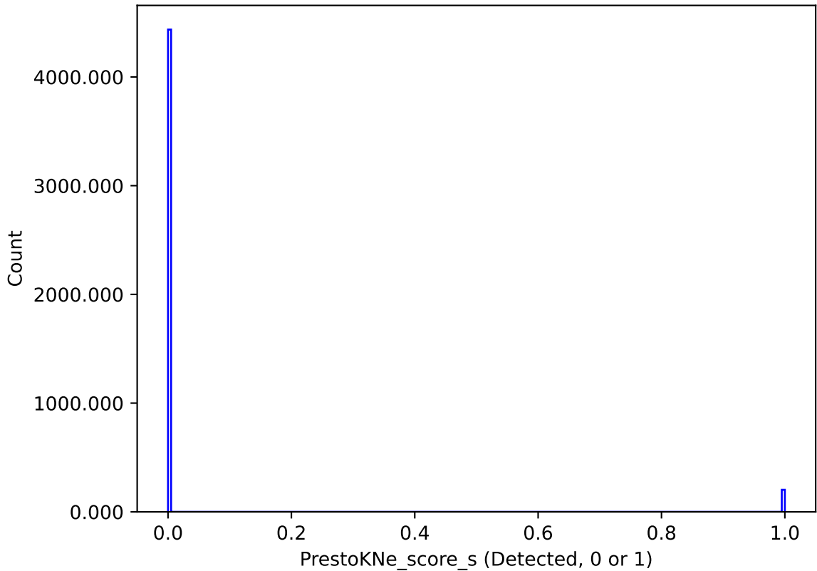
early_ss_template_fpextra1.5_v3.4_10yrs : PrestoKNe_score_s
