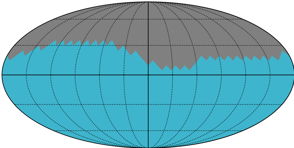
early_ss_template_fpextra1.5_v3.4_10yrs dm 20 interval 30 RRc Year 1-2: PeriodicStarModulationMetric
