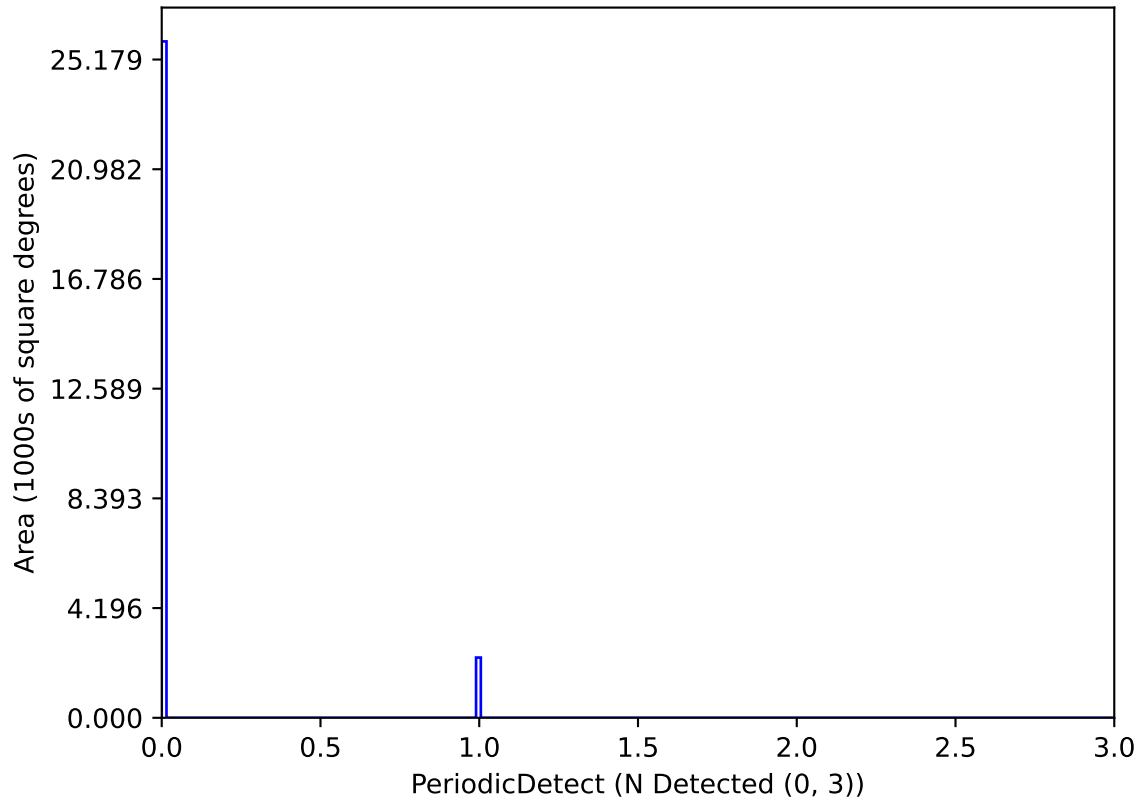
early_ss_template_fpextra1.5_v3.4_10yrs P_1.0_Mag_24_Amp_0.05-0.1-1: PeriodicDetect
